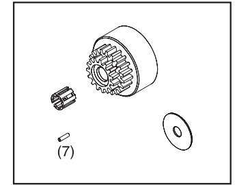
PD0644 2-SPEED CLUTCH BELL
