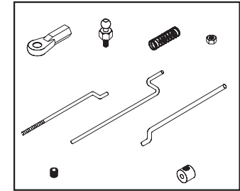
PD6084 THROTTLE / BRAKE LINKAGE
