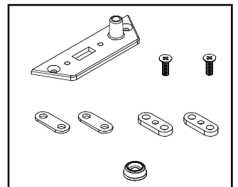
PD9091 SWITCH PLATE & SPACERS 開關盒蓋&墊片組
